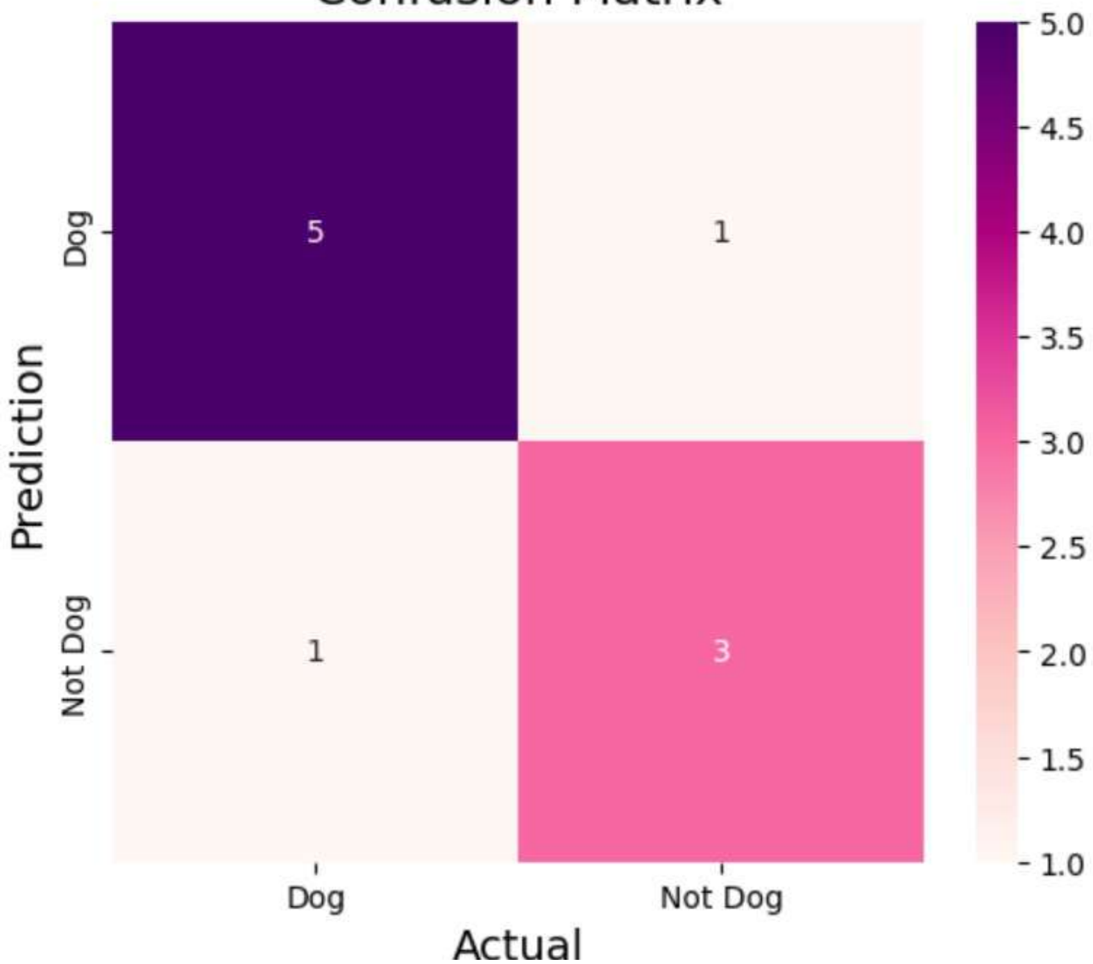
Confusion Matrix
